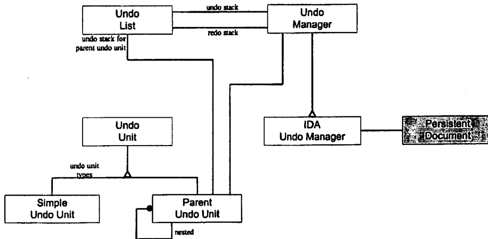
Figure 57 - Undo Manager Object Model
